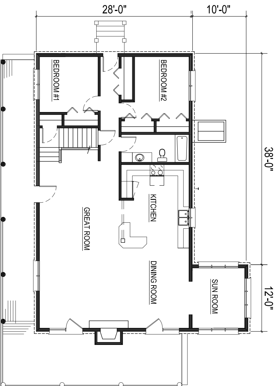
FIRST FLOOR
