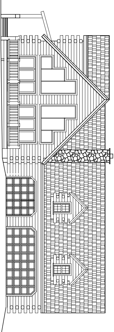
FRONT ELEVATION
