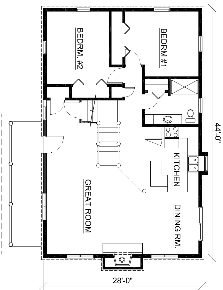
FIRST FLOOR
