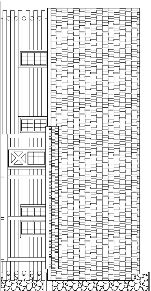
FRONT ELEVATION
