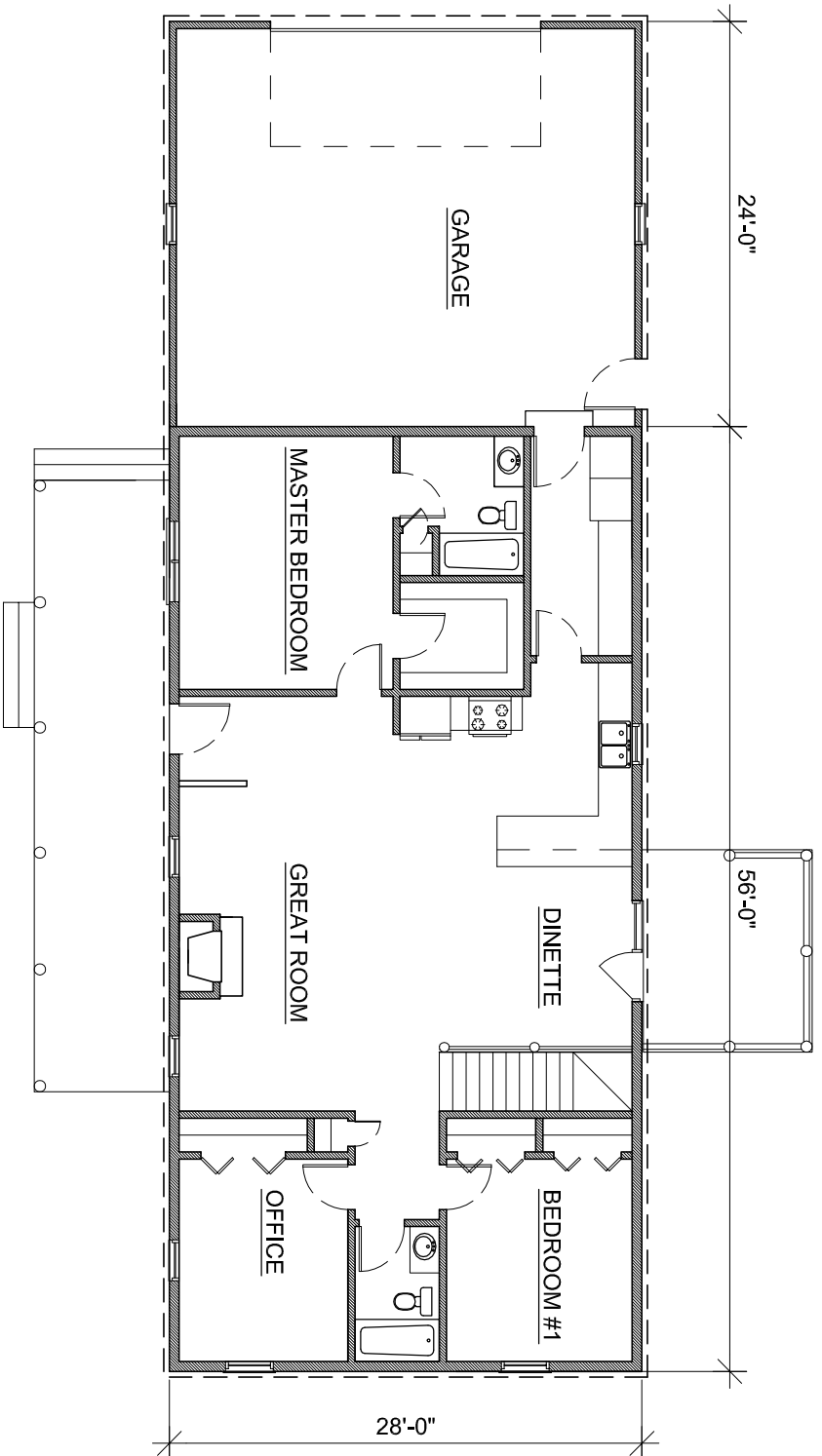
FIRST FLOOR
