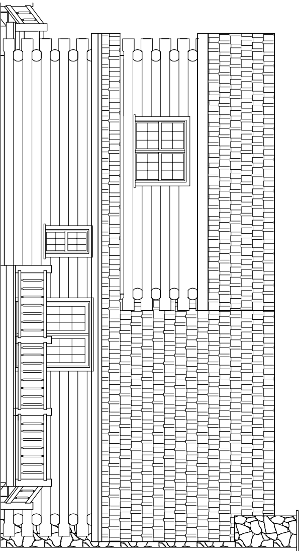
SIDE ELEVATION
