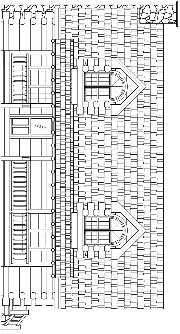
FRONT ELEVATION
