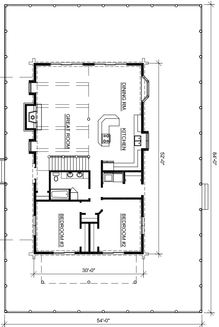
FIRST FLOOR
