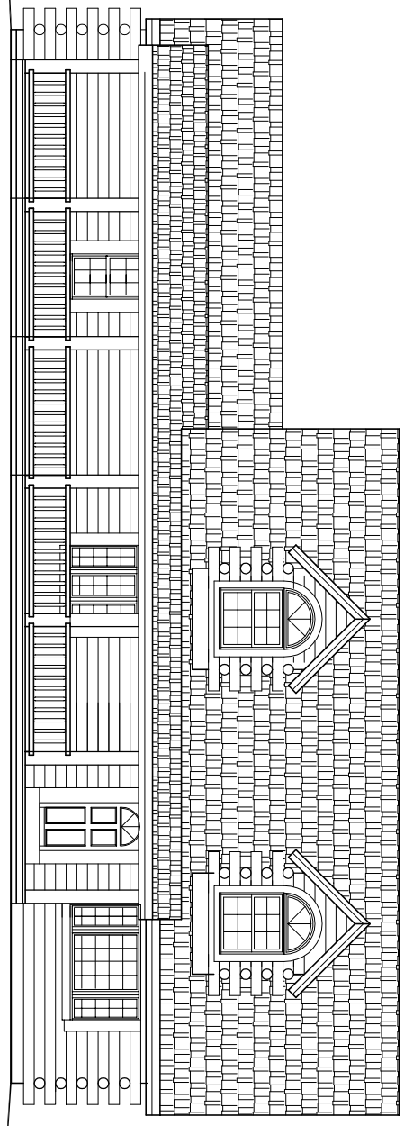
FRONT ELEVATION
